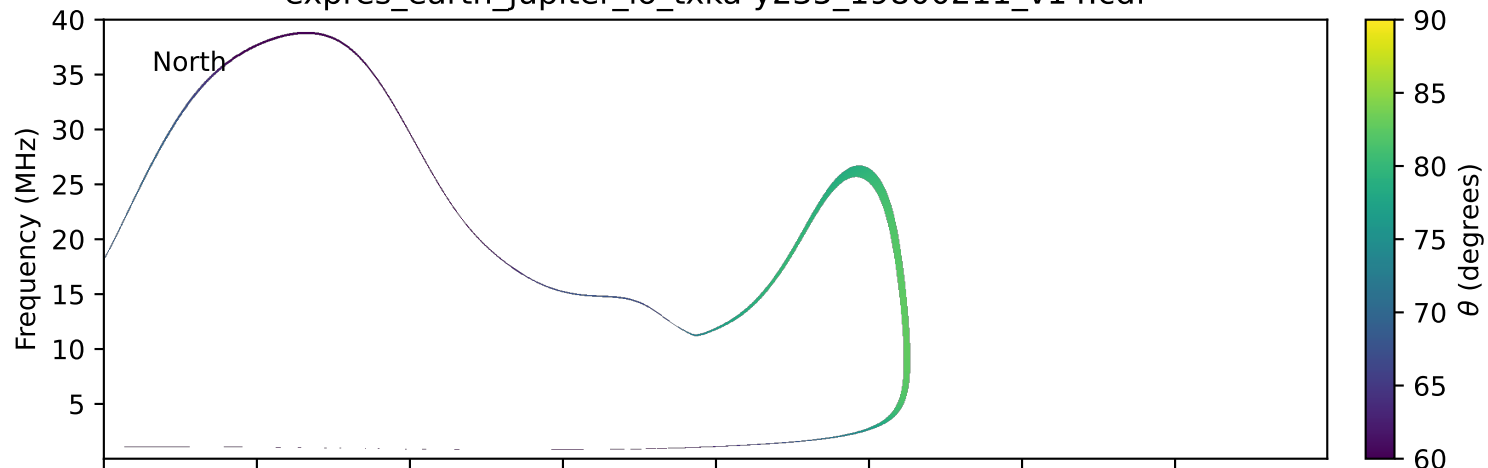
expres_earth_jupiter_io_txka-y235_19800211_v14.cdf
