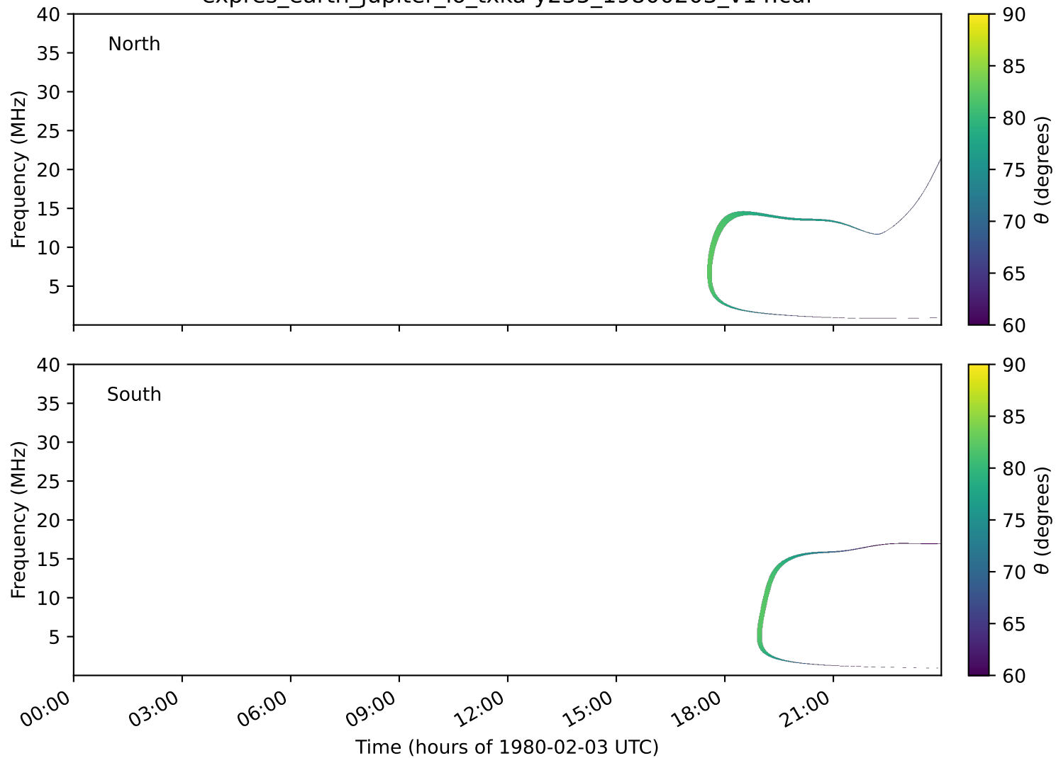
expres_earth_jupiter_io_txka-y235_19800203_v14.cdf
