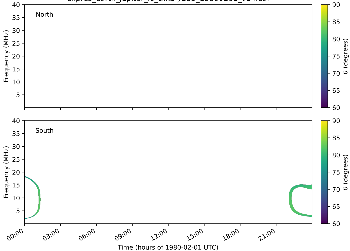
expres_earth_jupiter_io_txka-y235_19800201_v14.cdf
