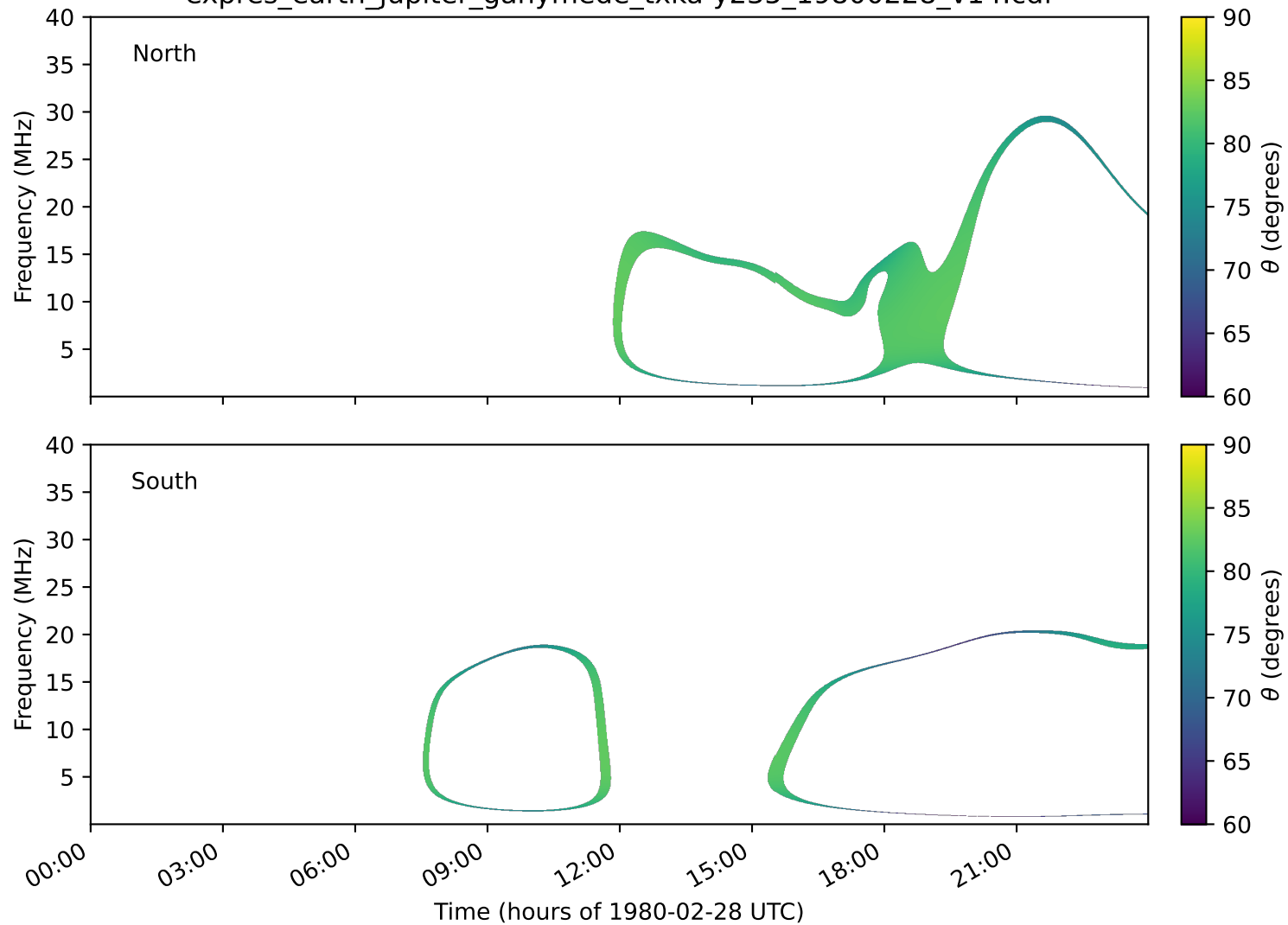
expres_earth_jupiter_ganymede_txka-y235_19800228_v14.cdf
