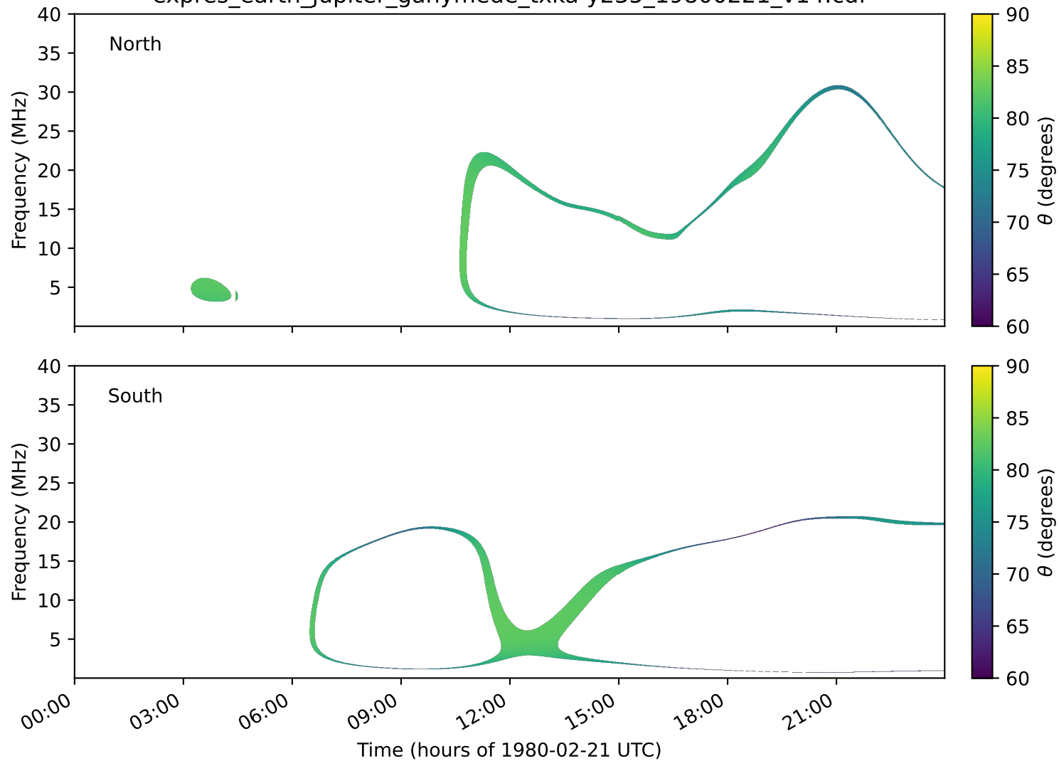
expres_earth_jupiter_ganymede_txka-y235_19800221_v14.cdf
