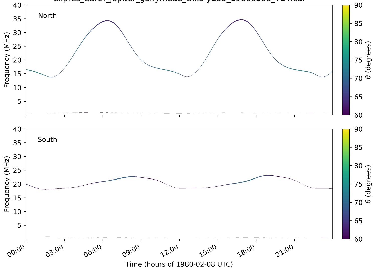
expres_earth_jupiter_ganymede_txka-y235_19800208_v14.cdf
