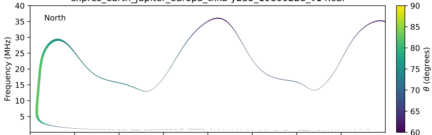
expres_earth_jupiter_europa_txka-y235_19800228_v14.cdf
