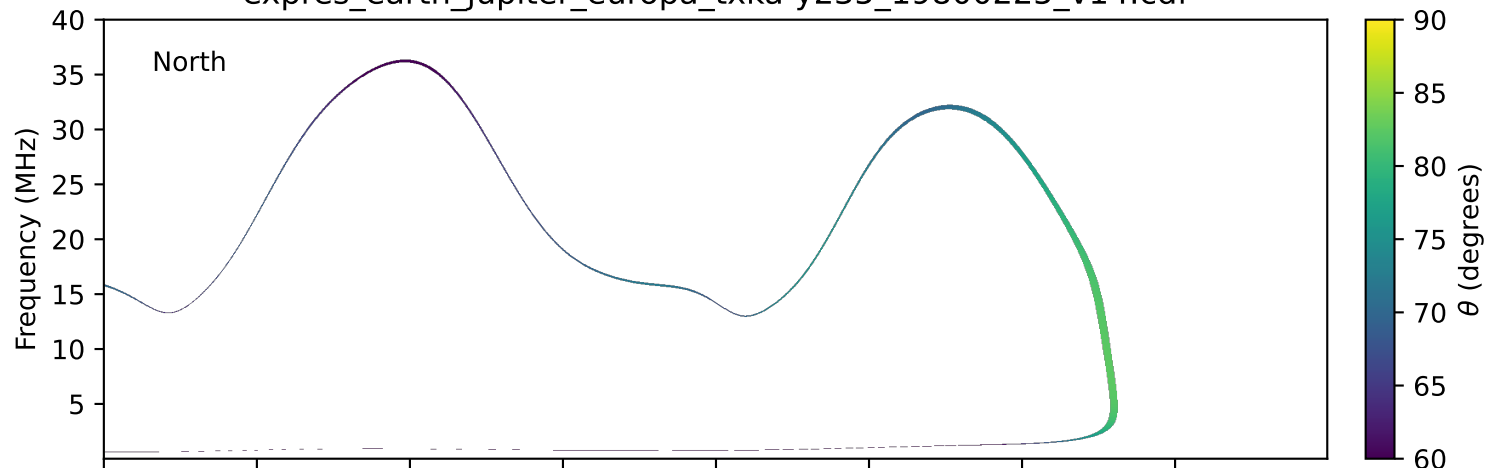
expres_earth_jupiter_europa_txka-y235_19800225_v14.cdf
