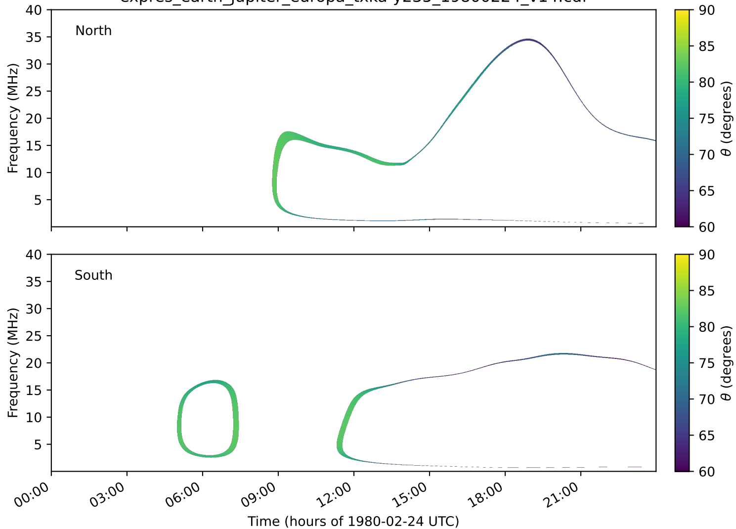
expres_earth_jupiter_europa_txka-y235_19800224_v14.cdf
