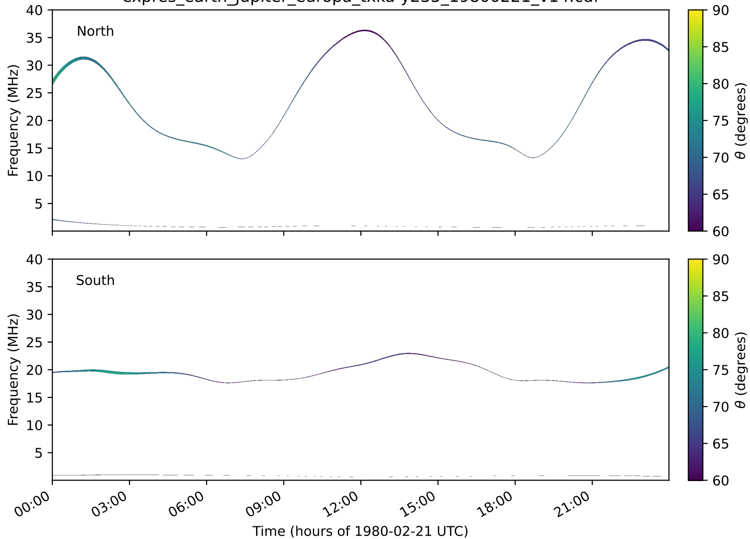
expres_earth_jupiter_europa_txka-y235_19800221_v14.cdf
