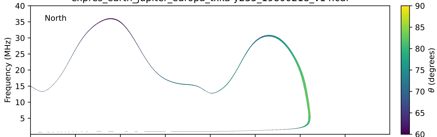
expres_earth_jupiter_europa_txka-y235_19800218_v14.cdf
