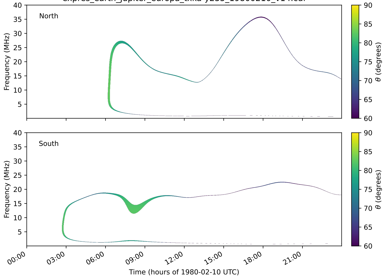
expres_earth_jupiter_europa_txka-y235_19800210_v14.cdf
