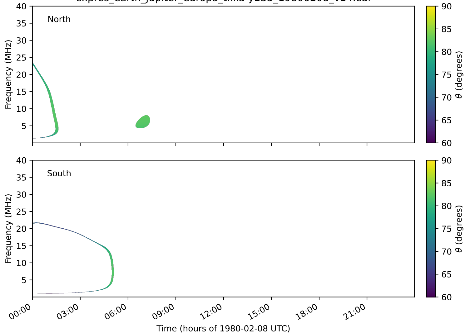
expres_earth_jupiter_europa_txka-y235_19800208_v14.cdf
