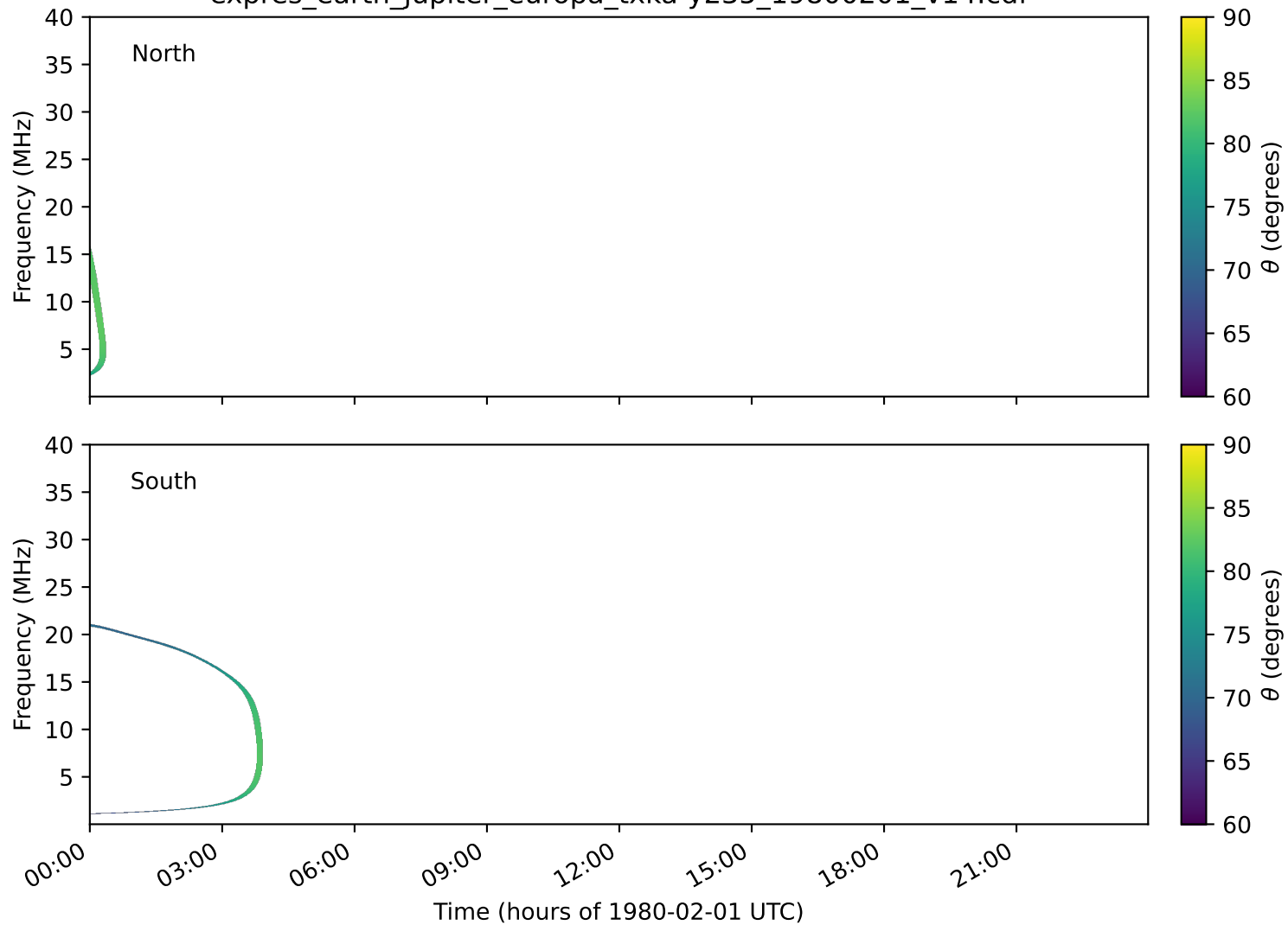
expres_earth_jupiter_europa_txka-y235_19800201_v14.cdf
