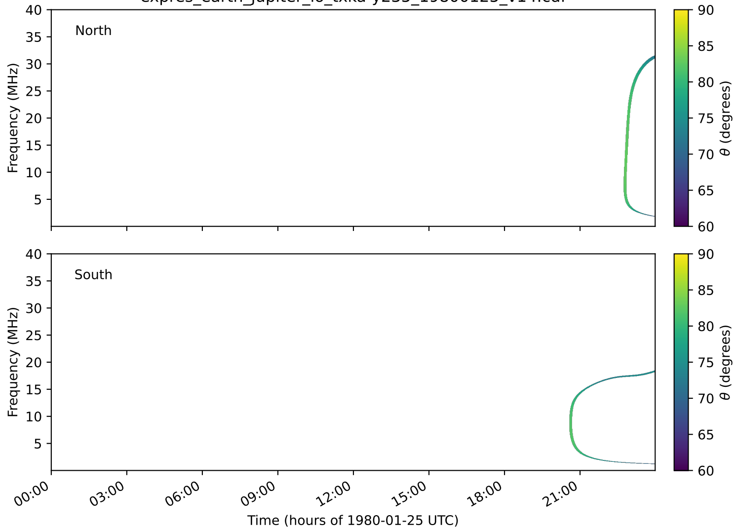
expres_earth_jupiter_io_txka-y235_19800125_v14.cdf
