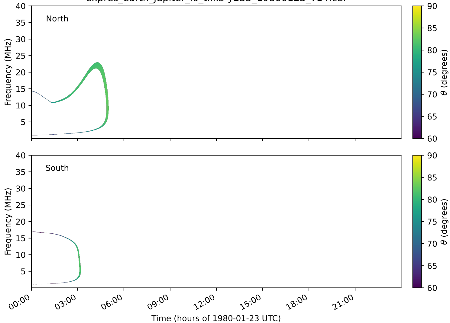
expres_earth_jupiter_io_txka-y235_19800123_v14.cdf
