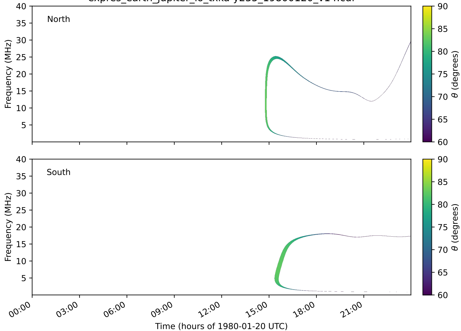
expres_earth_jupiter_io_txka-y235_19800120_v14.cdf
