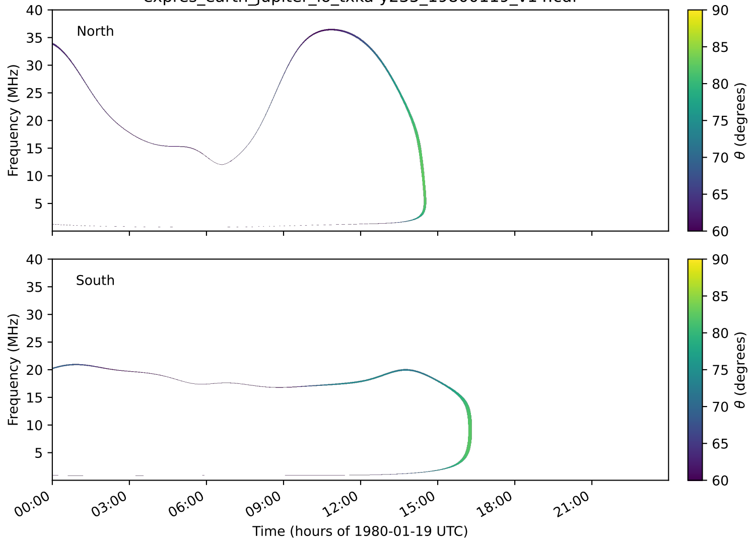
expres_earth_jupiter_io_txka-y235_19800119_v14.cdf
