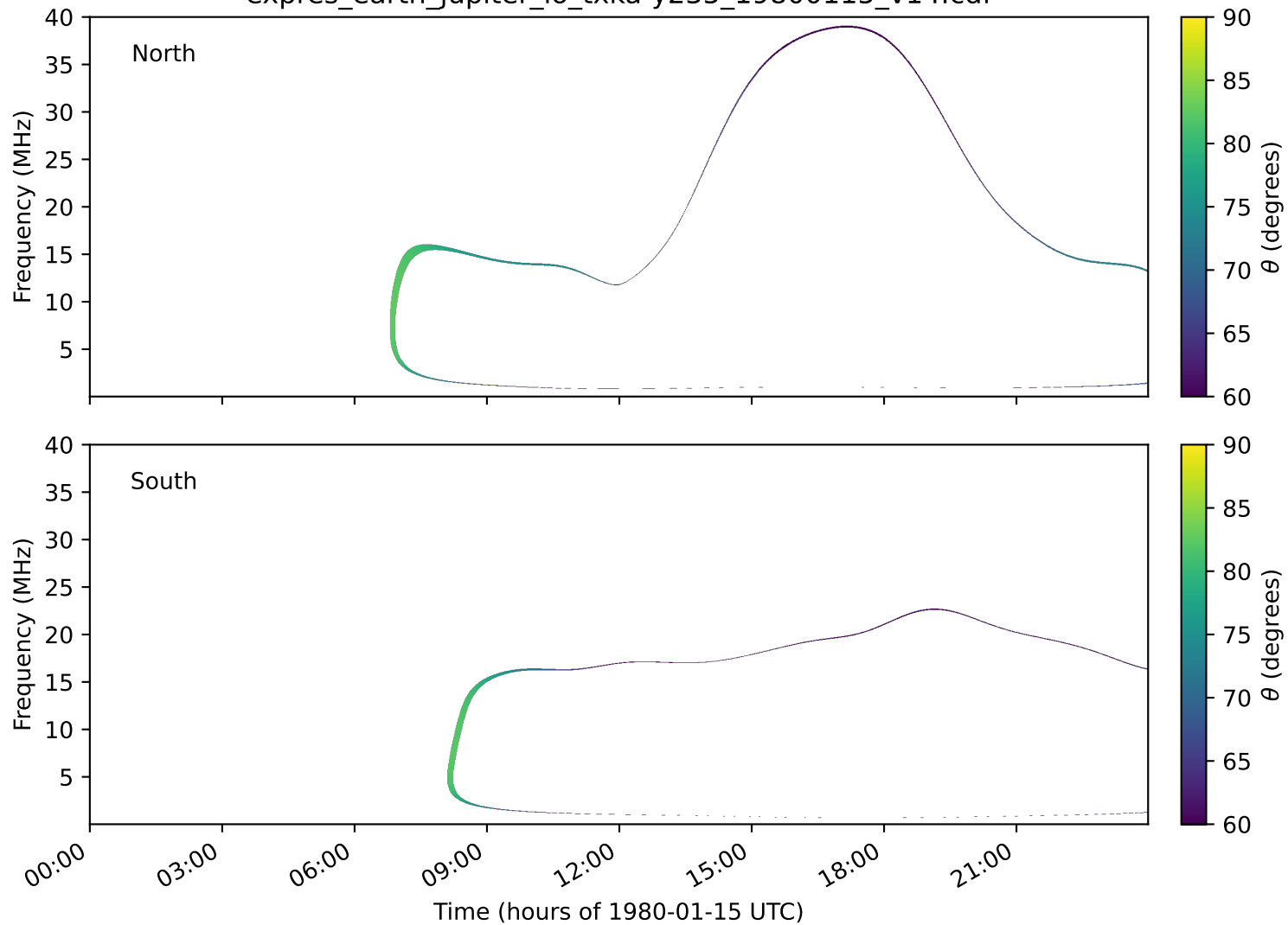
expres_earth_jupiter_io_txka-y235_19800115_v14.cdf
