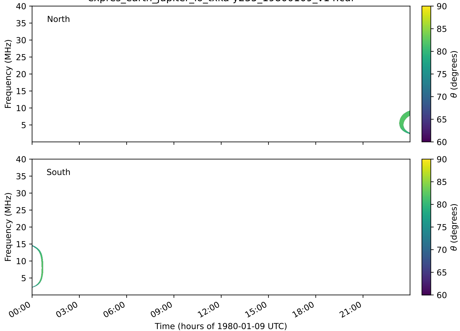
expres_earth_jupiter_io_txka-y235_19800109_v14.cdf
