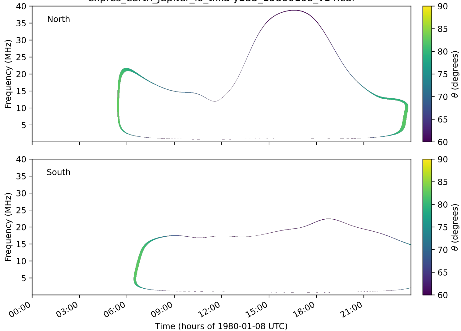
expres_earth_jupiter_io_txka-y235_19800108_v14.cdf
