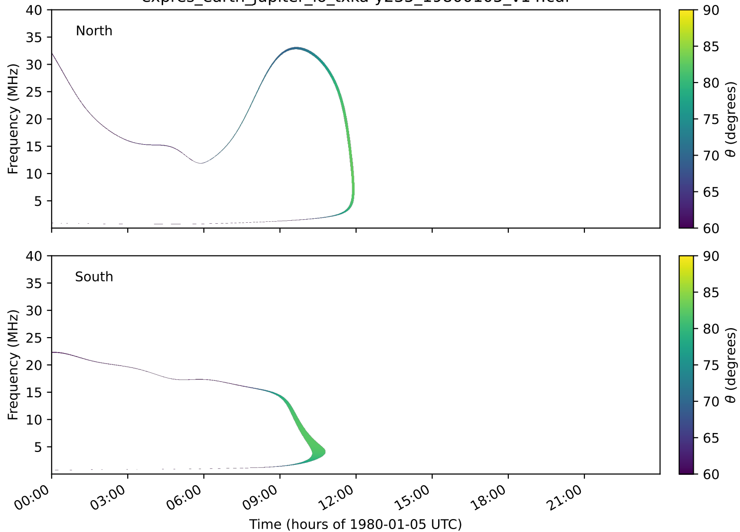
expres_earth_jupiter_io_txka-y235_19800105_v14.cdf
