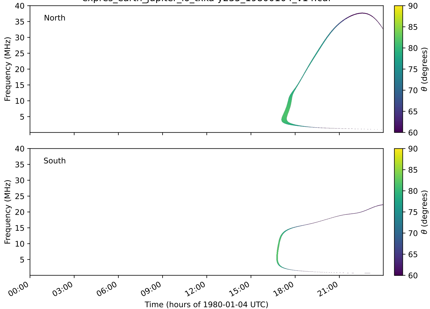
expres_earth_jupiter_io_txka-y235_19800104_v14.cdf
