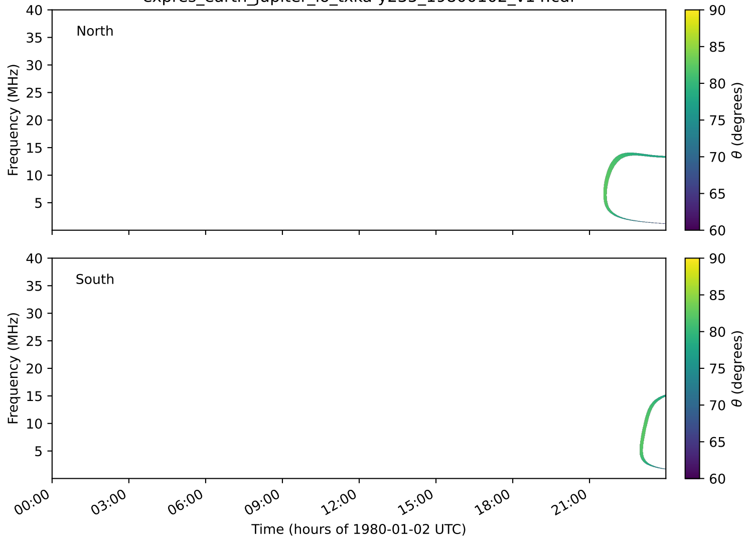
expres_earth_jupiter_io_txka-y235_19800102_v14.cdf
