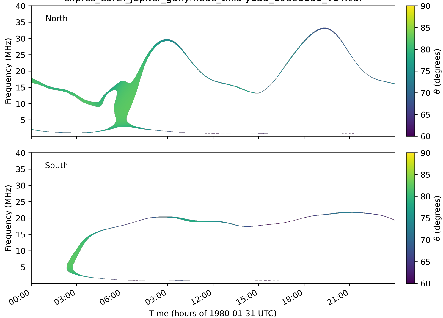
expres_earth_jupiter_ganymede_txka-y235_19800131_v14.cdf
