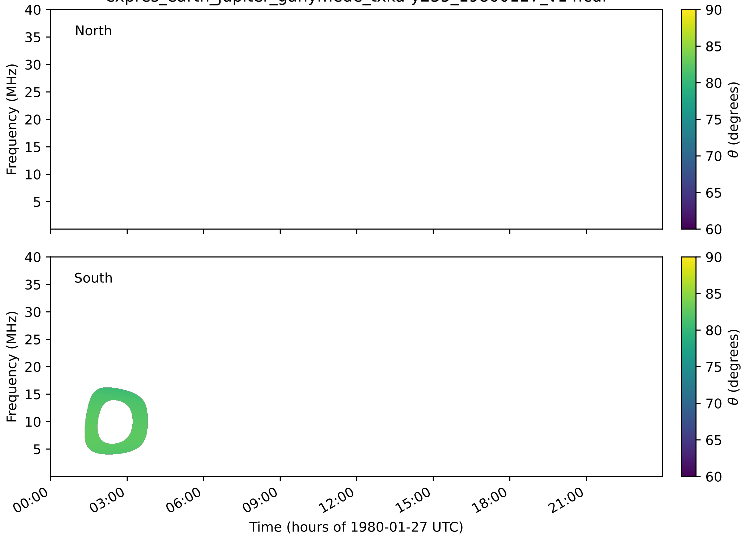
expres_earth_jupiter_ganymede_txka-y235_19800127_v14.cdf
