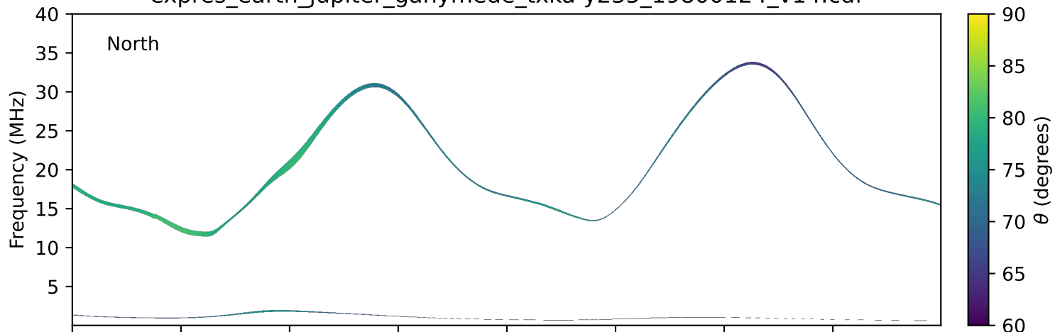
expres_earth_jupiter_ganymede_txka-y235_19800124_v14.cdf
