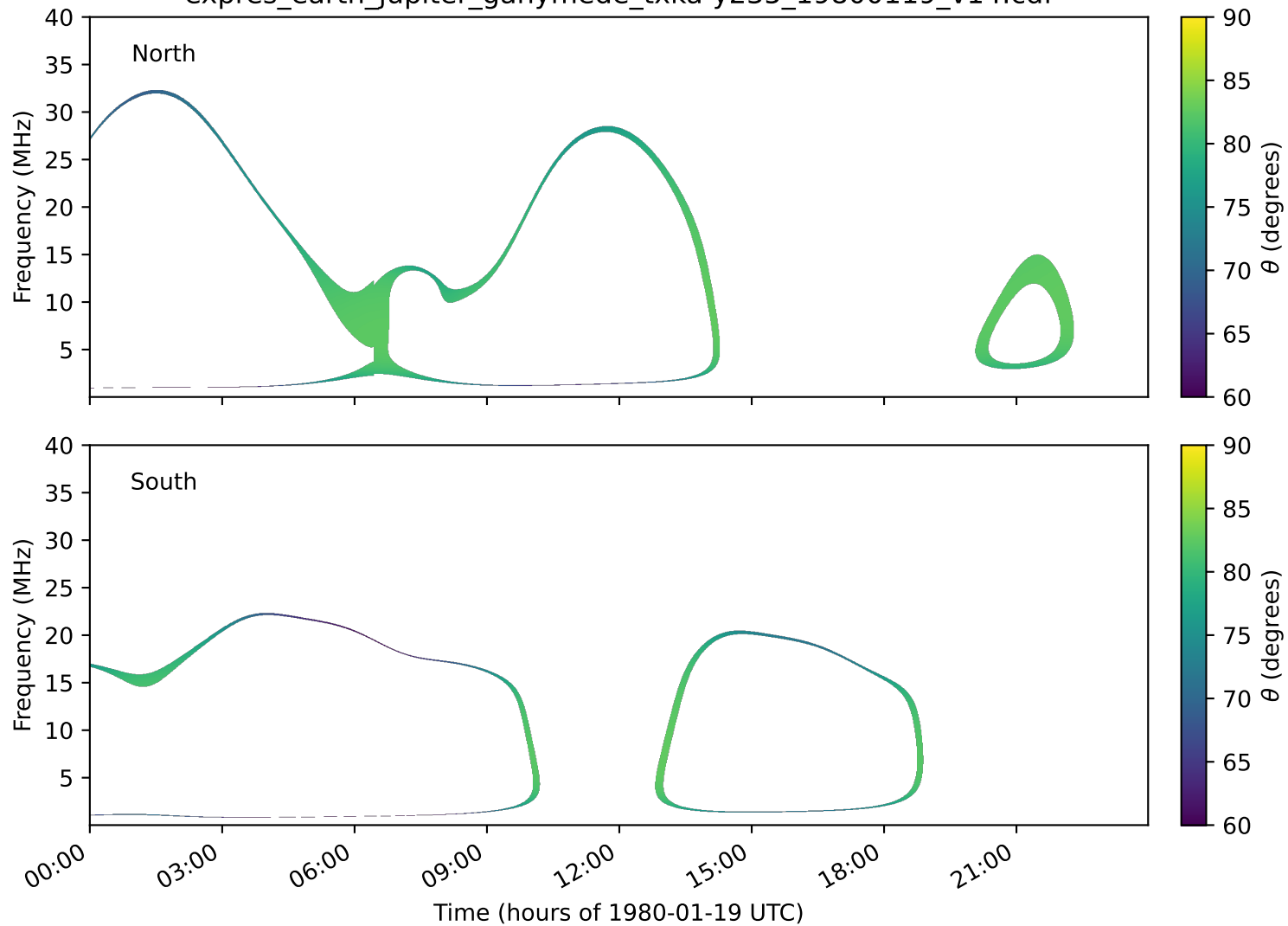
expres_earth_jupiter_ganymede_txka-y235_19800119_v14.cdf
