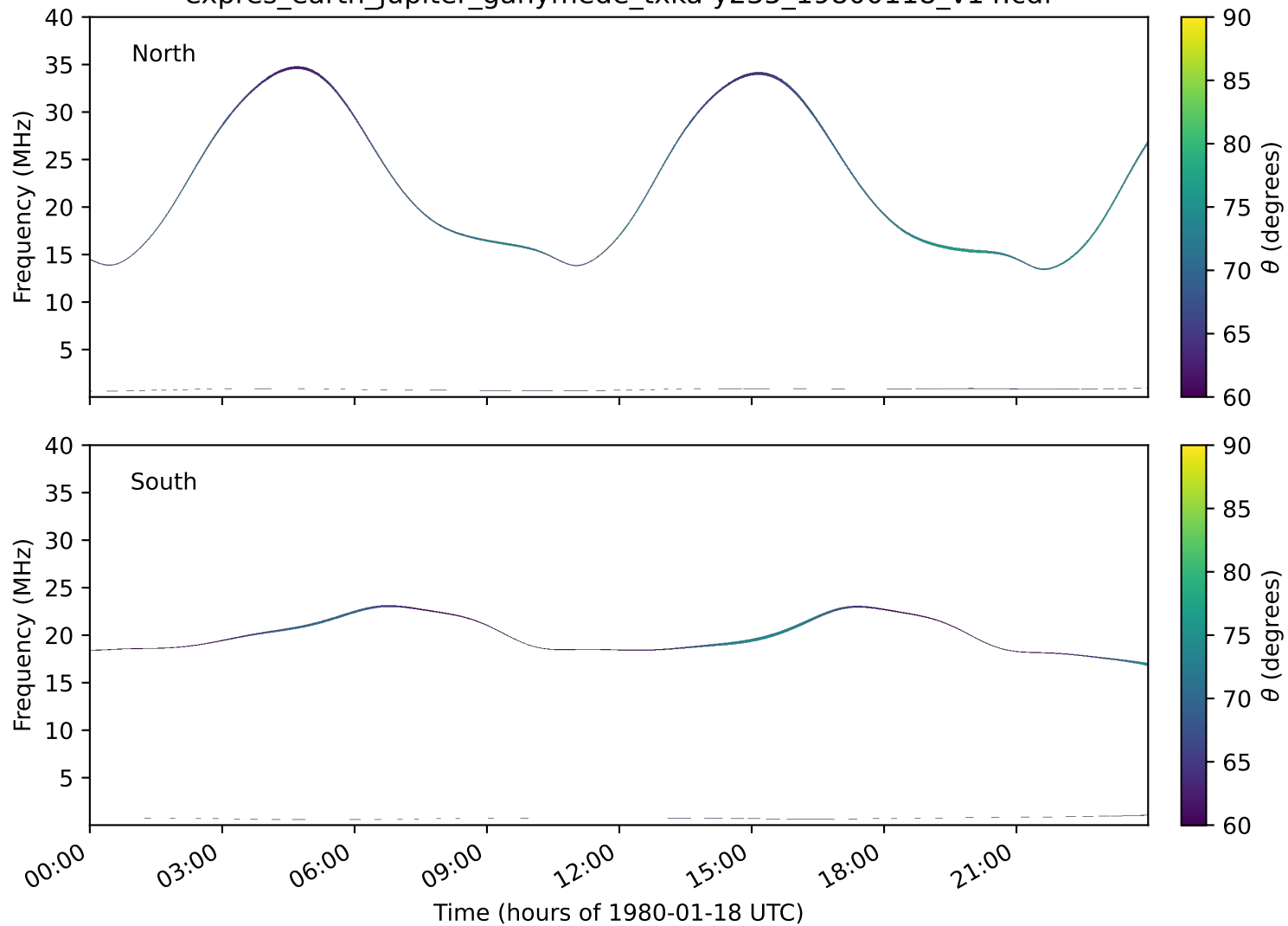
expres_earth_jupiter_ganymede_txka-y235_19800118_v14.cdf
