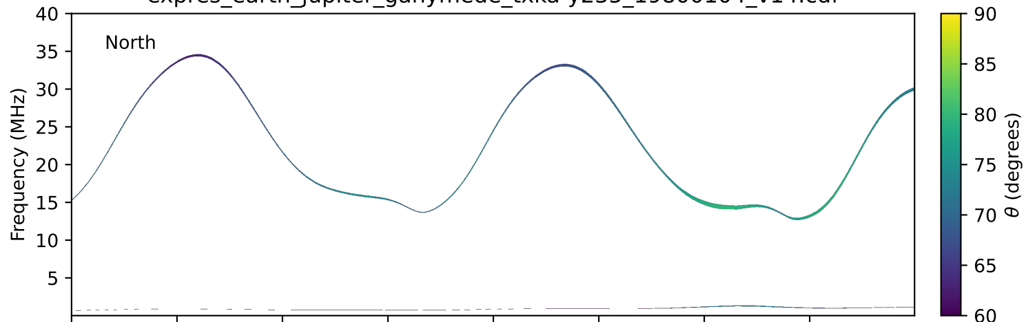
expres_earth_jupiter_ganymede_txka-y235_19800104_v14.cdf
