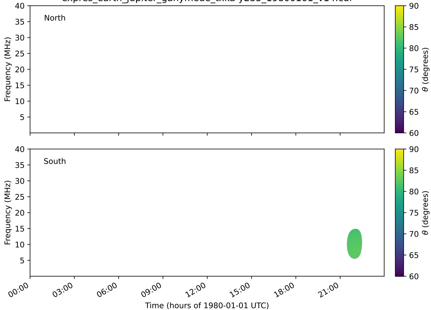
expres_earth_jupiter_ganymede_txka-y235_19800101_v14.cdf
