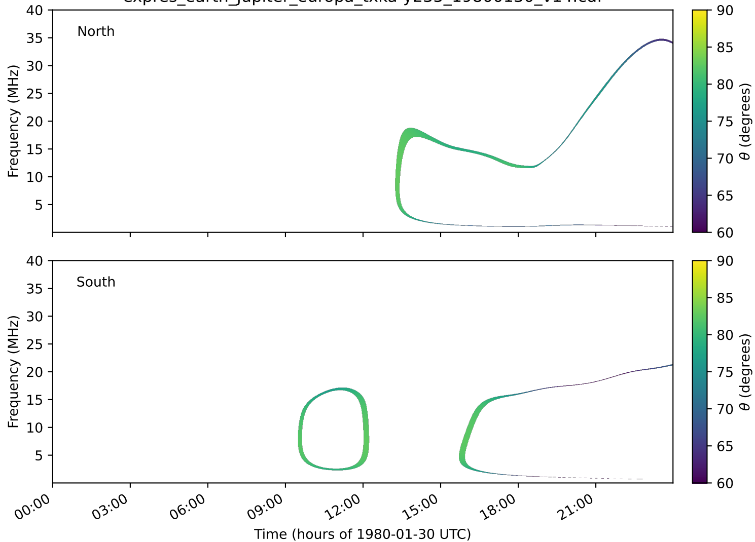
expres_earth_jupiter_europa_txka-y235_19800130_v14.cdf
