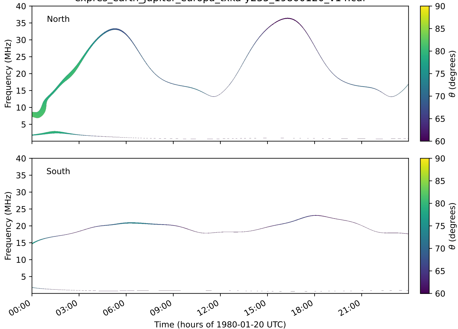
expres_earth_jupiter_europa_txka-y235_19800120_v14.cdf
