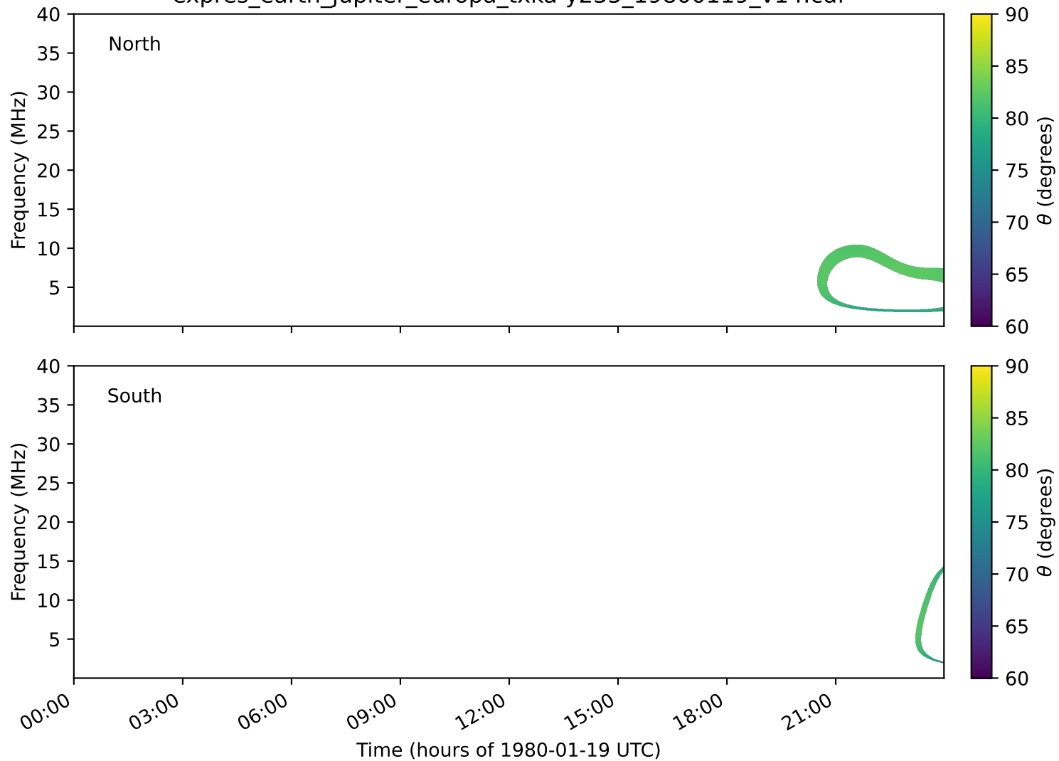
expres_earth_jupiter_europa_txka-y235_19800119_v14.cdf
