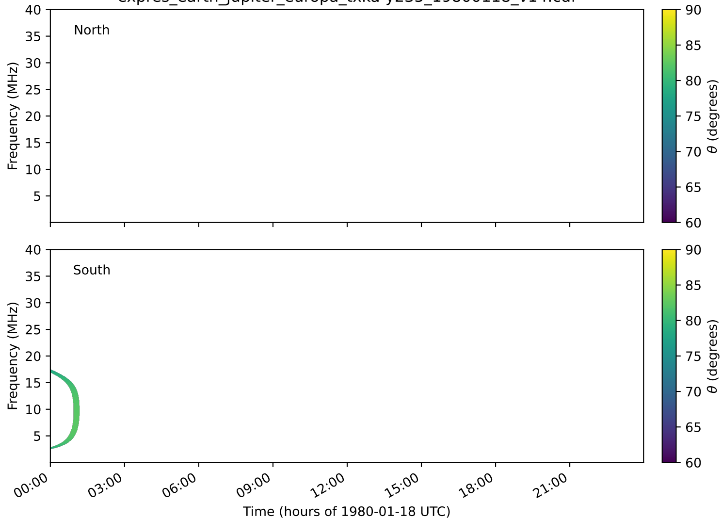
expres_earth_jupiter_europa_txka-y235_19800118_v14.cdf
