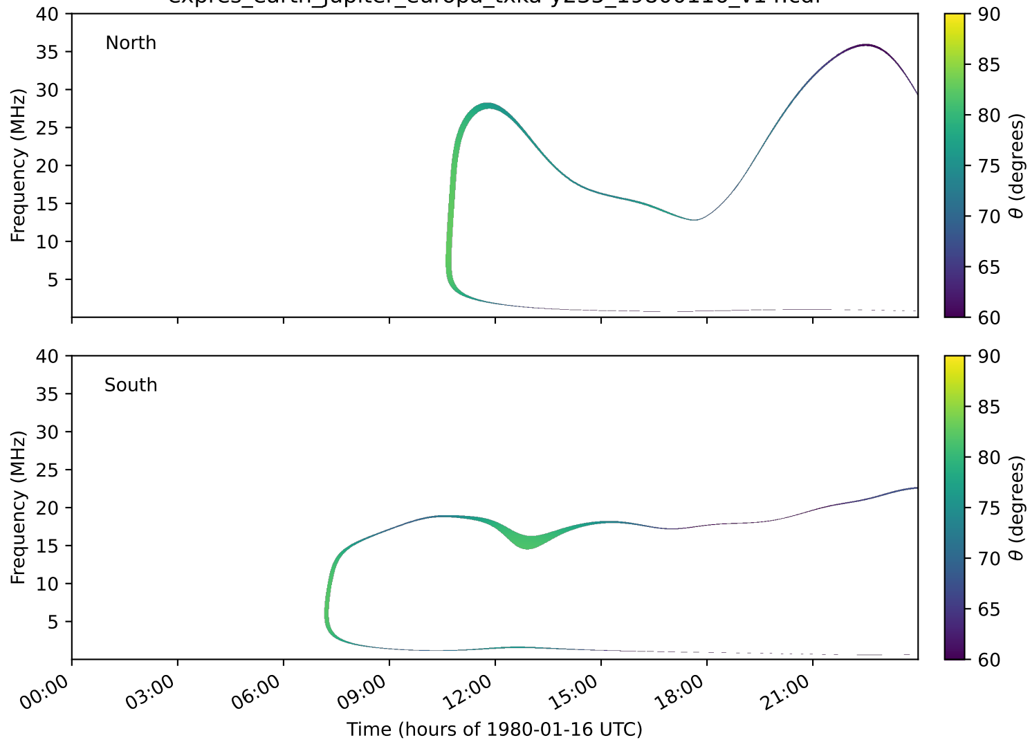
expres_earth_jupiter_europa_txka-y235_19800116_v14.cdf
