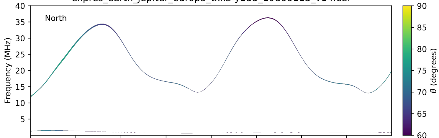
expres_earth_jupiter_europa_txka-y235_19800113_v14.cdf
