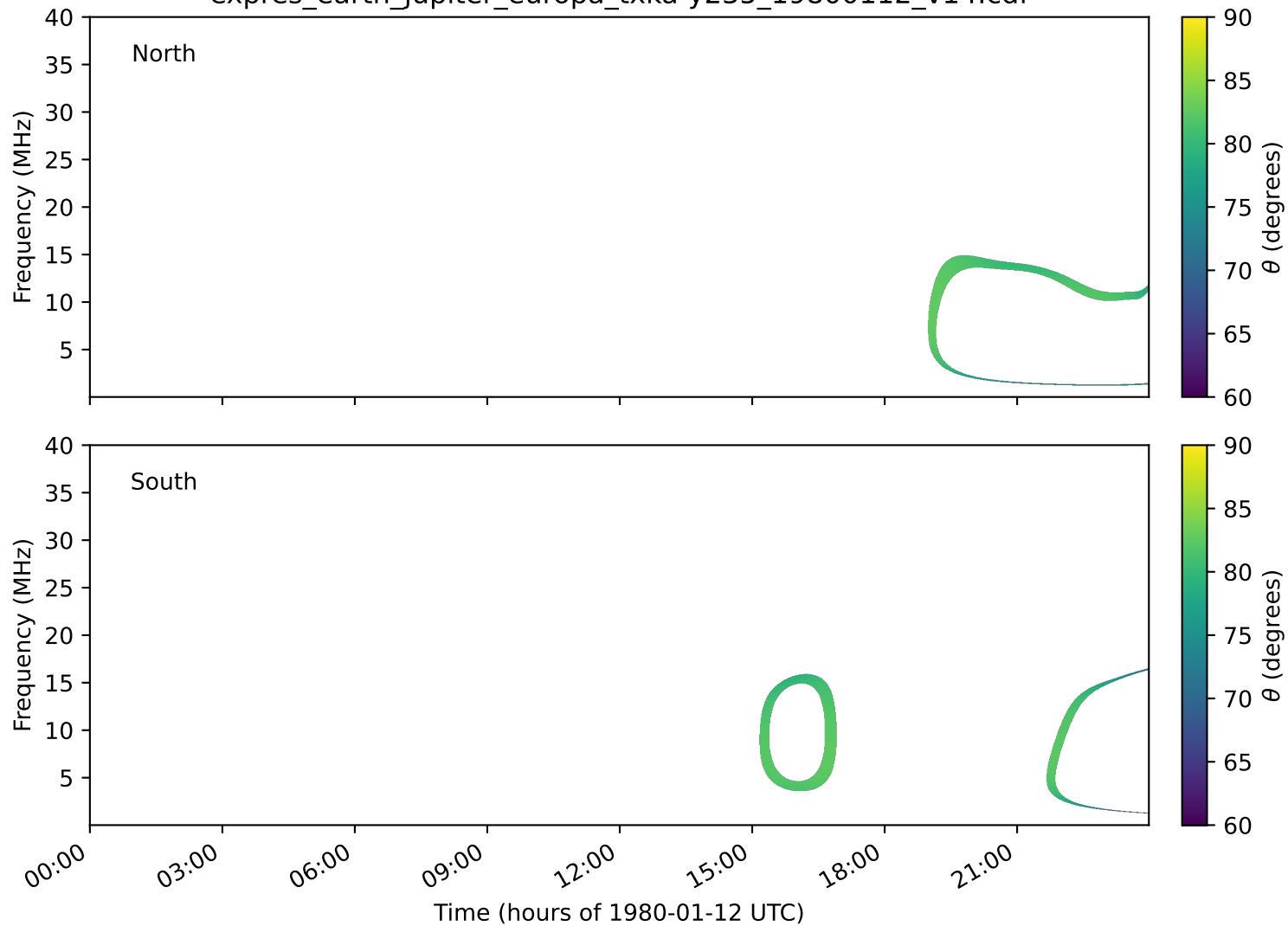
expres_earth_jupiter_europa_txka-y235_19800112_v14.cdf
