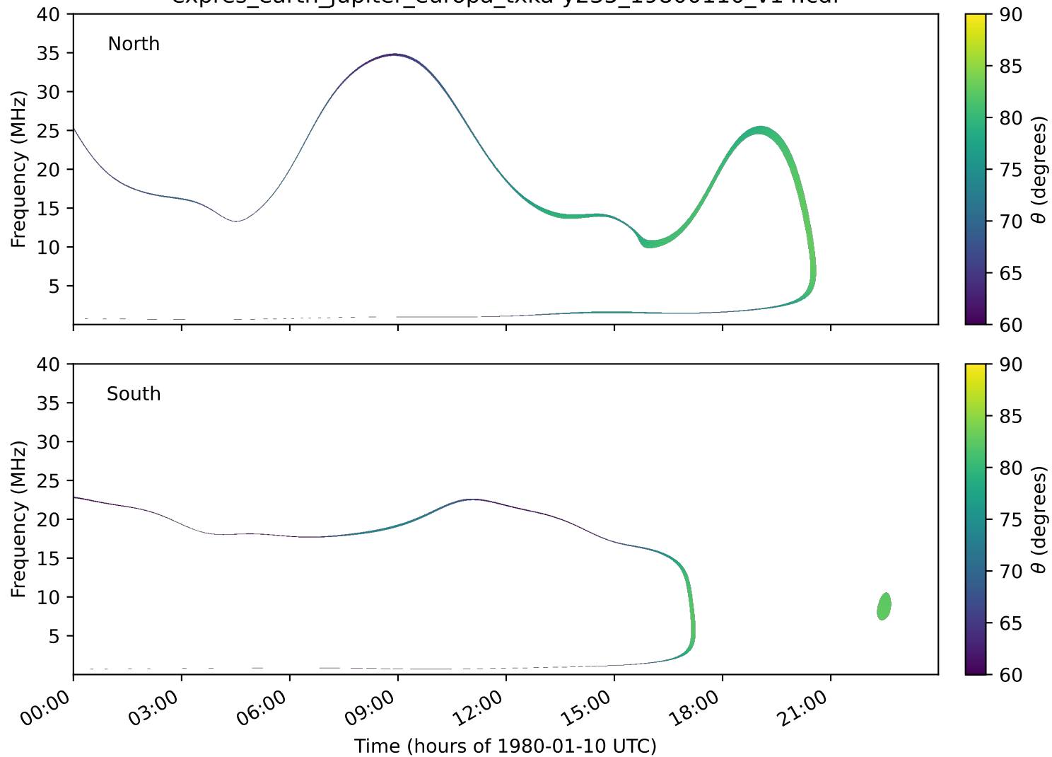
expres_earth_jupiter_europa_txka-y235_19800110_v14.cdf
