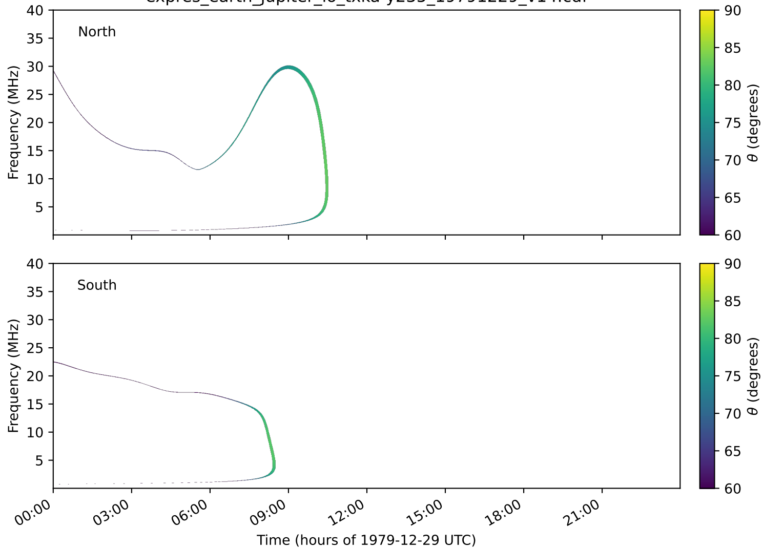
expres_earth_jupiter_io_txka-y235_19791229_v14.cdf
