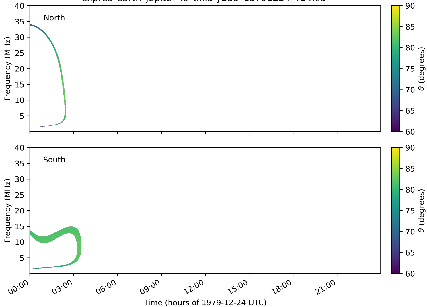
expres_earth_jupiter_io_txka-y235_19791224_v14.cdf
