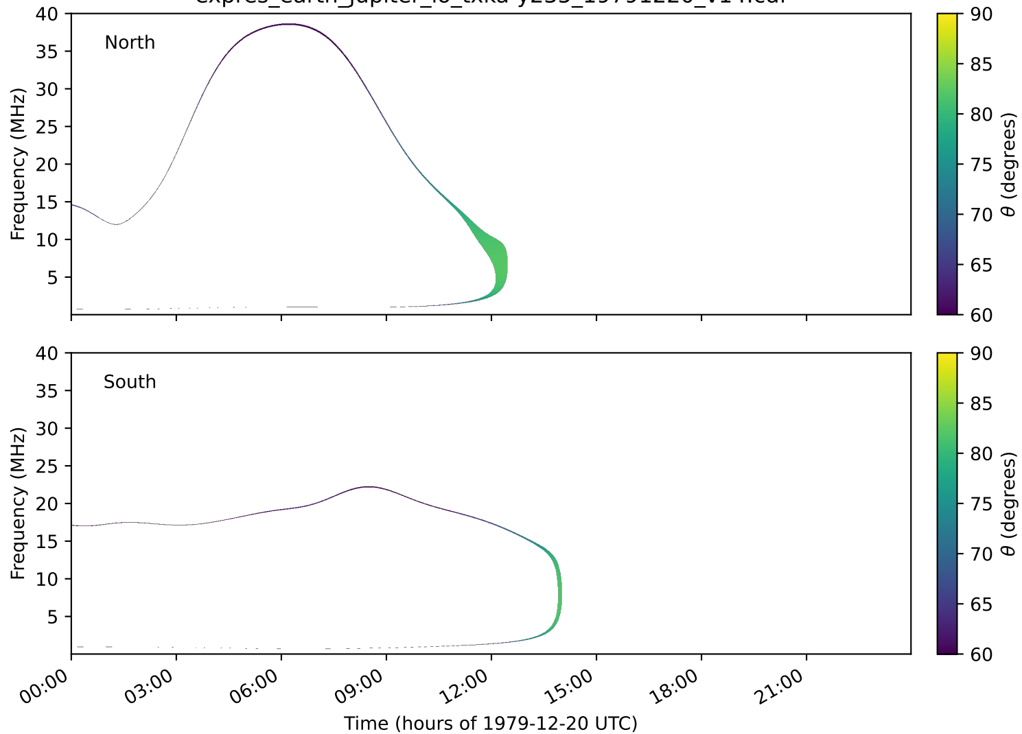
expres_earth_jupiter_io_txka-y235_19791220_v14.cdf
