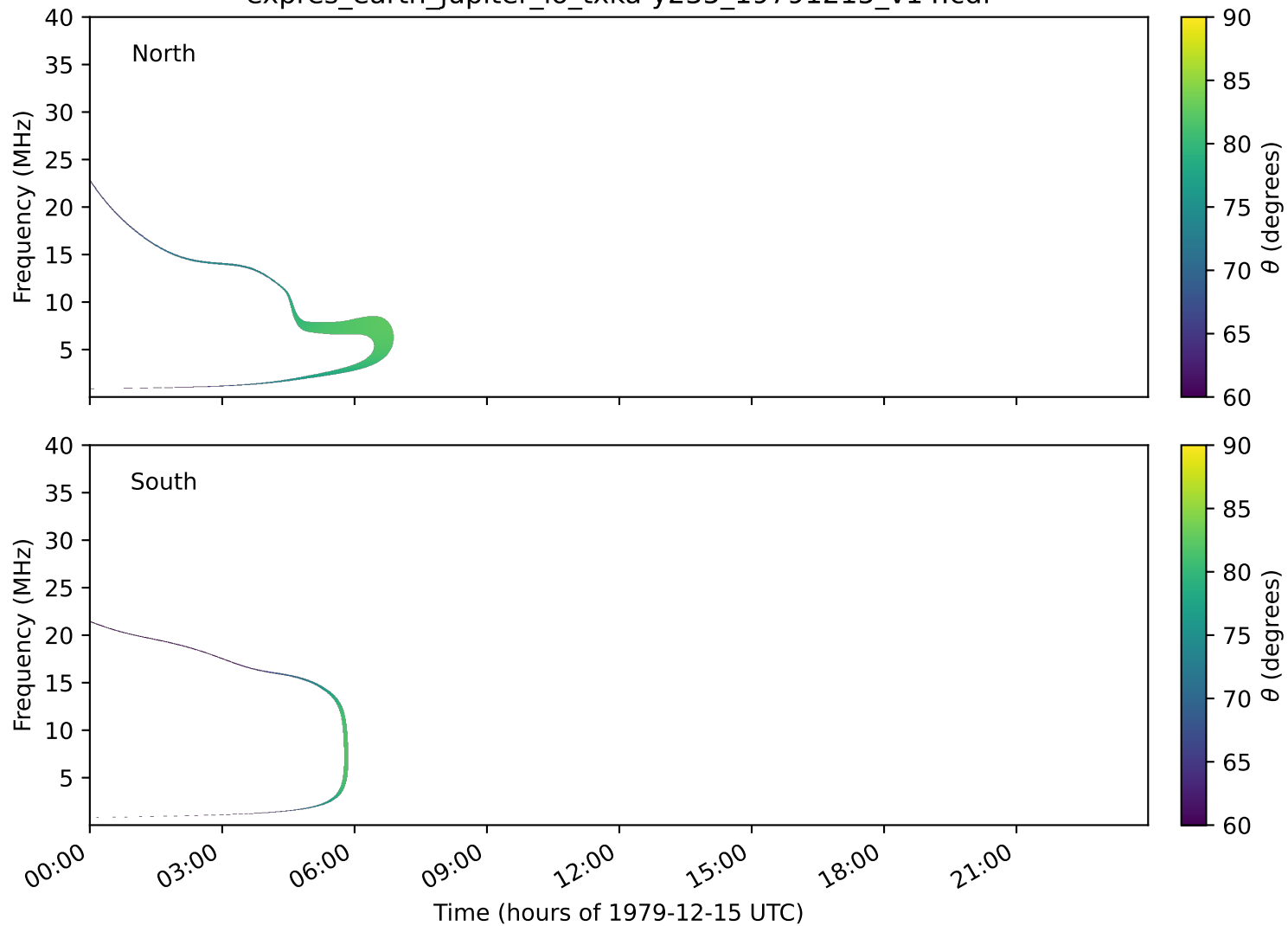
expres_earth_jupiter_io_txka-y235_19791215_v14.cdf
