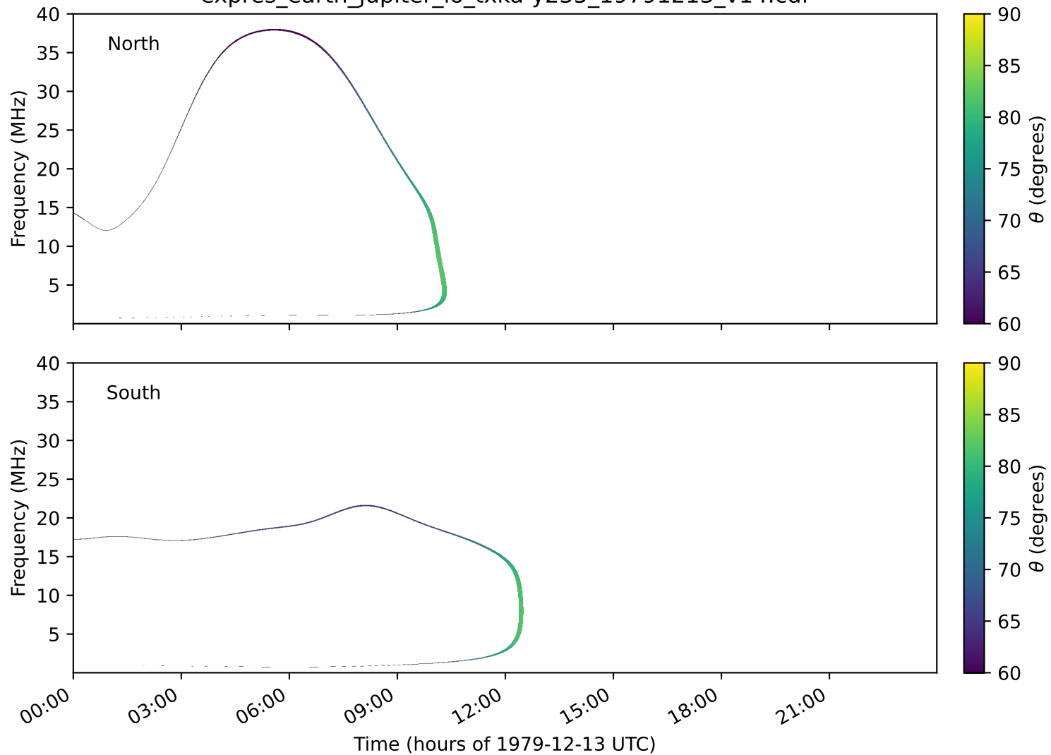
expres_earth_jupiter_io_txka-y235_19791213_v14.cdf
