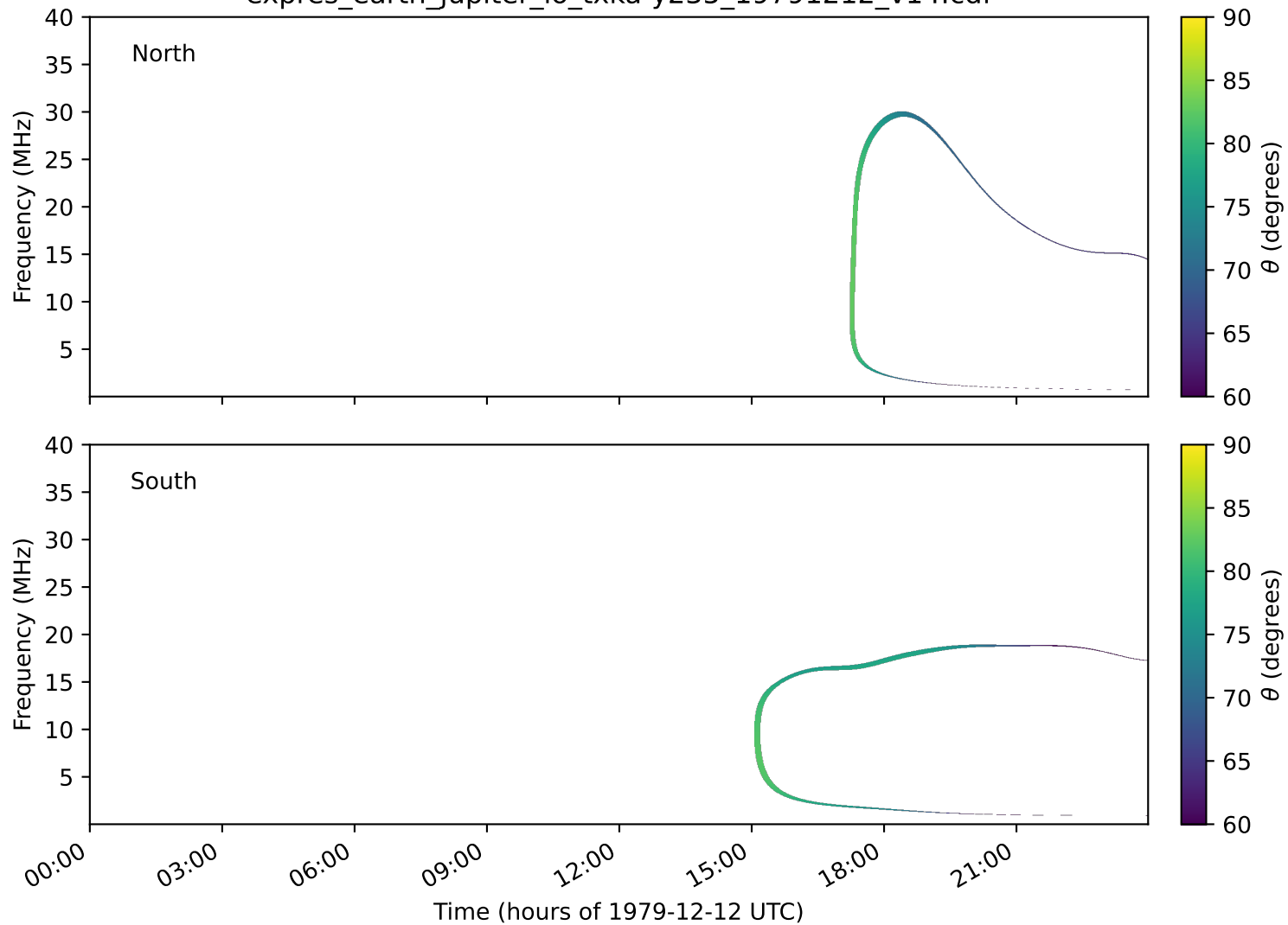
expres_earth_jupiter_io_txka-y235_19791212_v14.cdf
