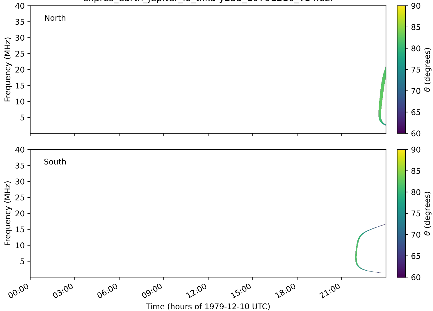
expres_earth_jupiter_io_txka-y235_19791210_v14.cdf
