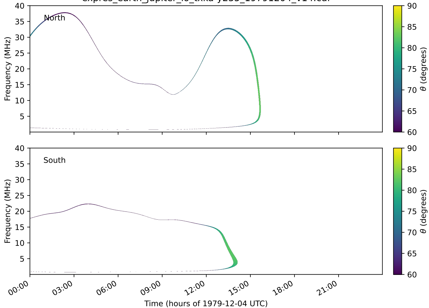
expres_earth_jupiter_io_txka-y235_19791204_v14.cdf
