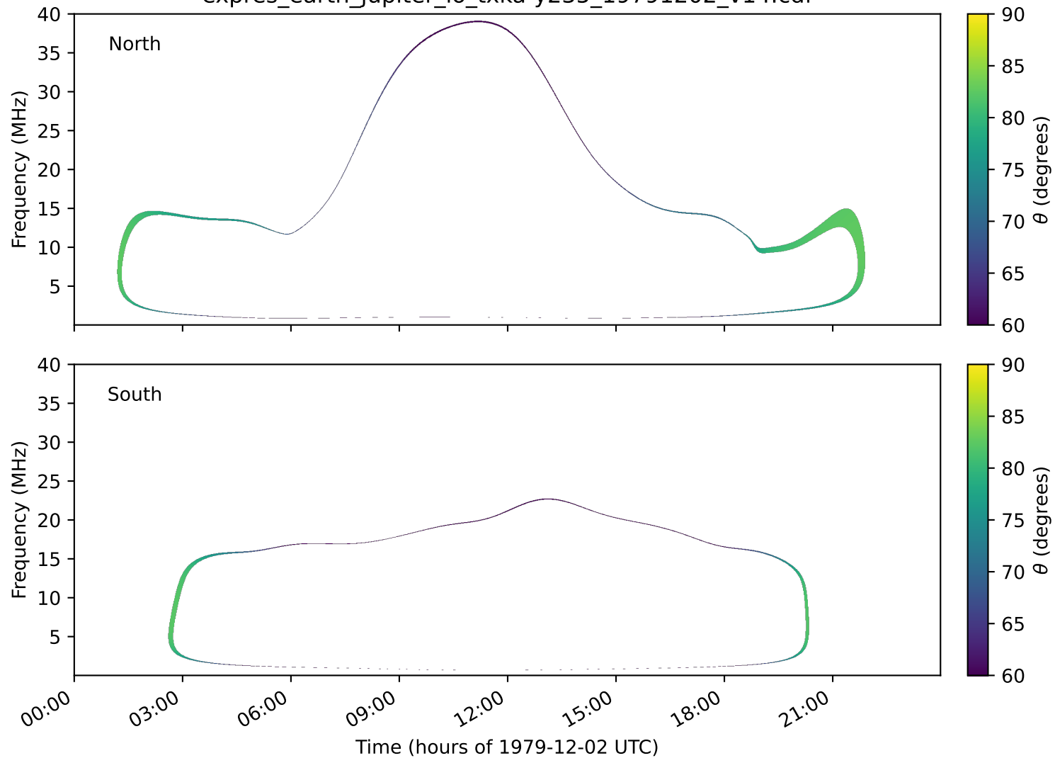
expres_earth_jupiter_io_txka-y235_19791202_v14.cdf
