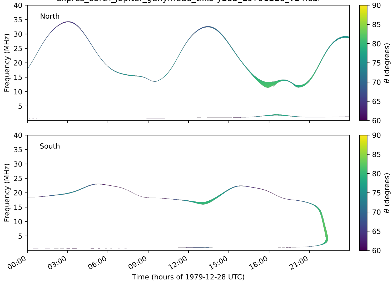
expres_earth_jupiter_ganymede_txka-y235_19791228_v14.cdf
