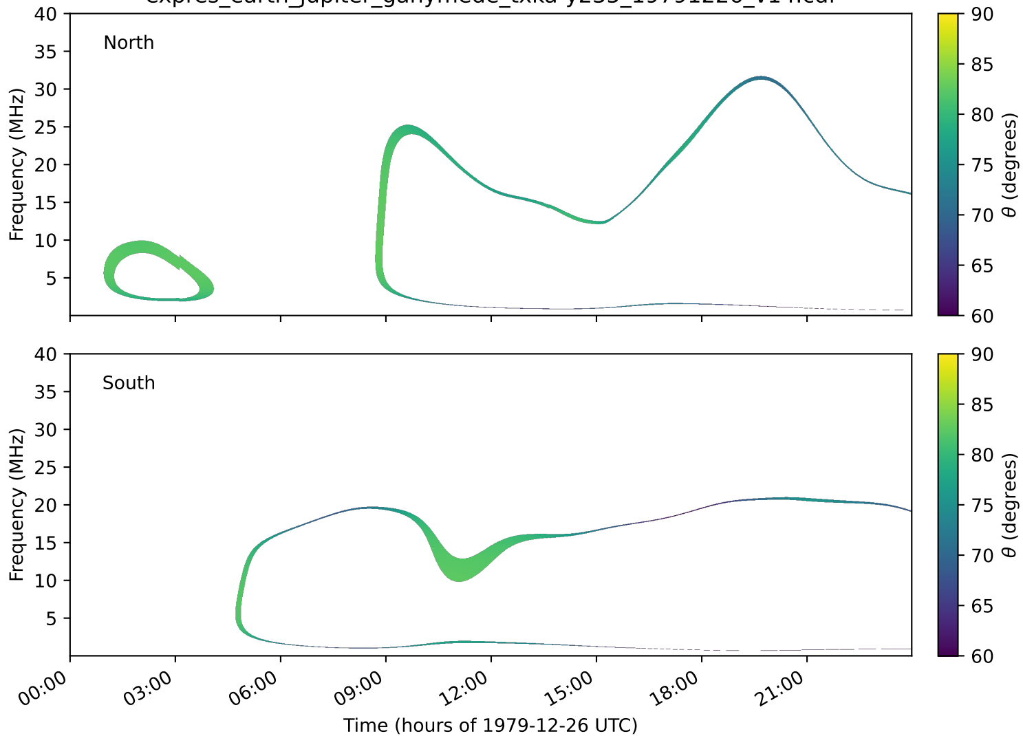
expres_earth_jupiter_ganymede_txka-y235_19791226_v14.cdf
